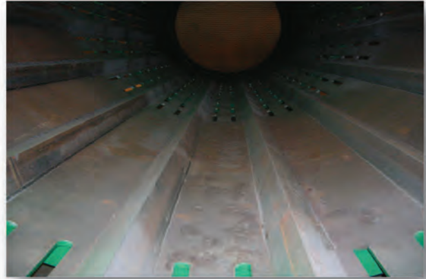
Lifters for this rugged equipment are installed with submerged arc welds to provide shell uniformity. They are also reverse steel angled.
