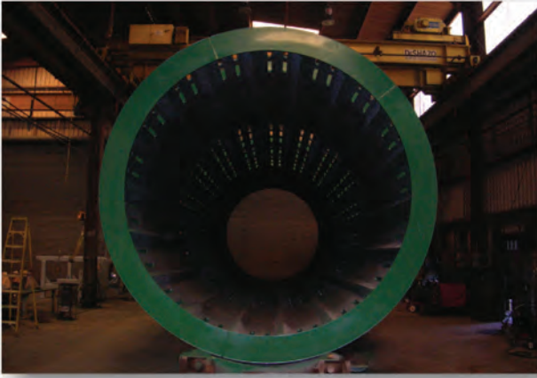
Drum debarkers fabricated in Fulghum's plant.
